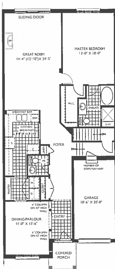
Ground Floor 1,506 sq.ft
