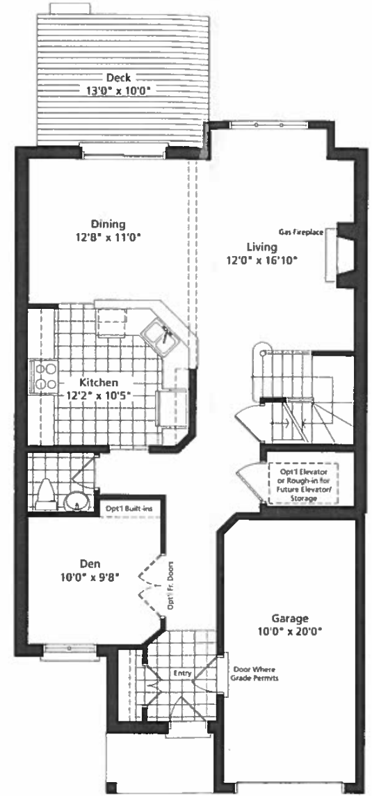
ALTERNATE MAIN FLOOR
